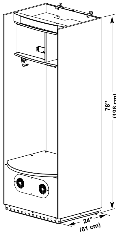
Straight Side Profile
