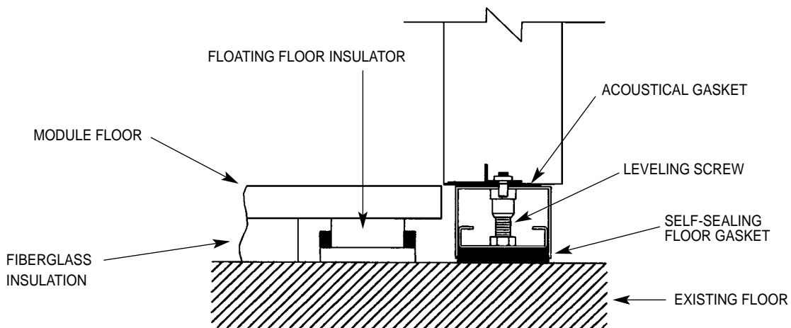
Typical wall cross section to existing floor.
