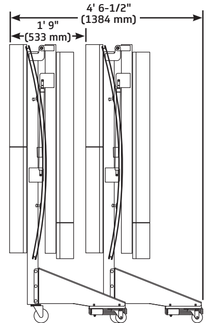
Nesting at 11' 6" (3505 mm) Height
