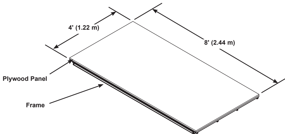
STRATA Plywood Deck, 4' x 8' (1.22x2.44 m)
