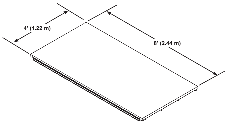
STRATA Finished Deck, 4' x 8' (1.22x2.44 m)
