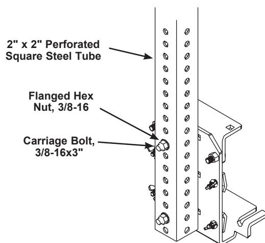
Example using Steel Tube
