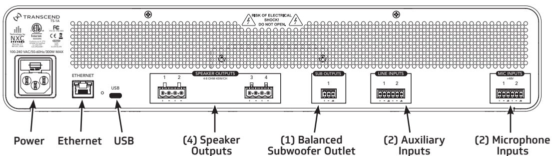
TS-1A Transcend Processor
