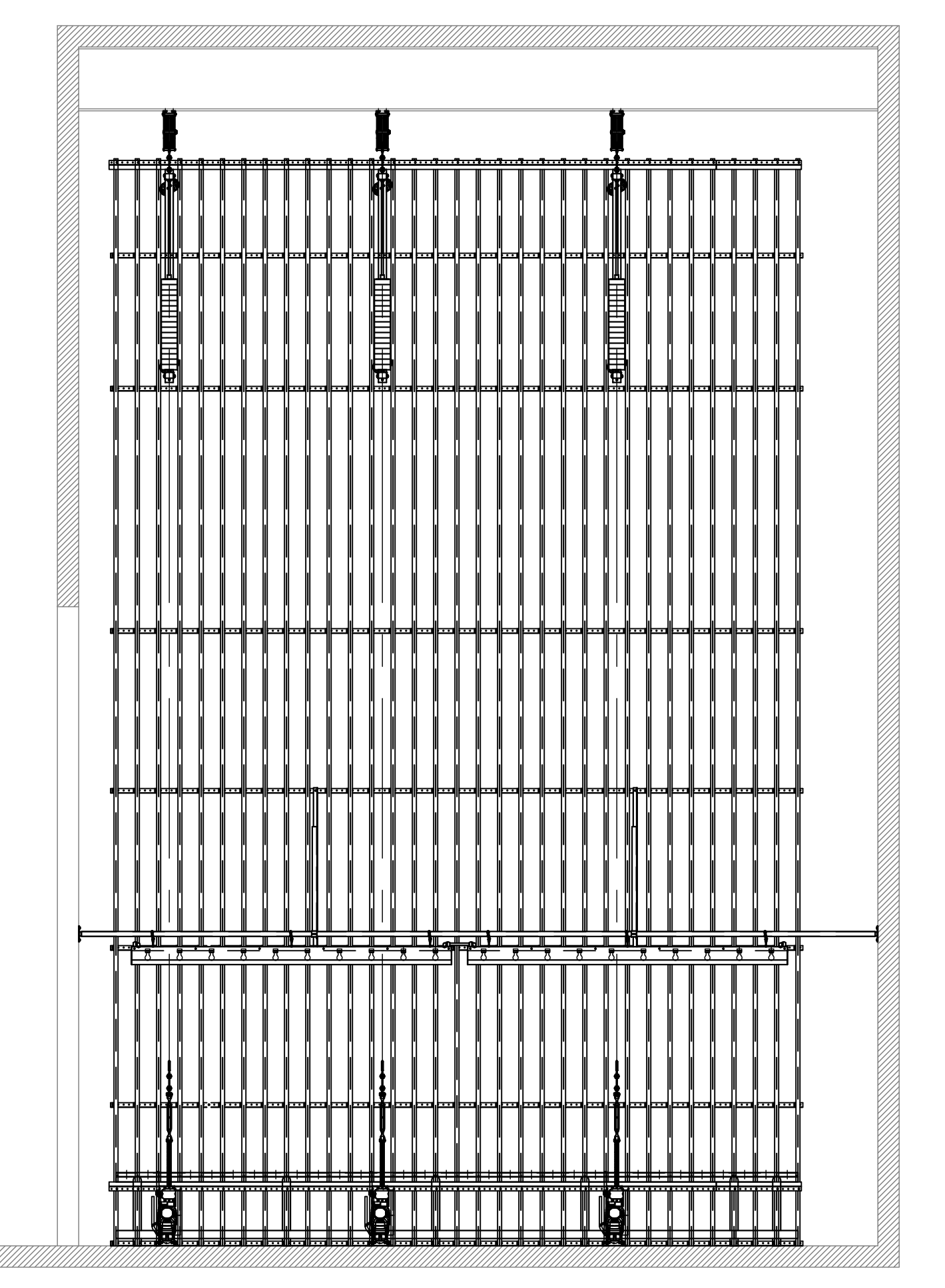
3 POWERASSIST SECTION PA-1 SCALE: 1/4" = 1'-0"
