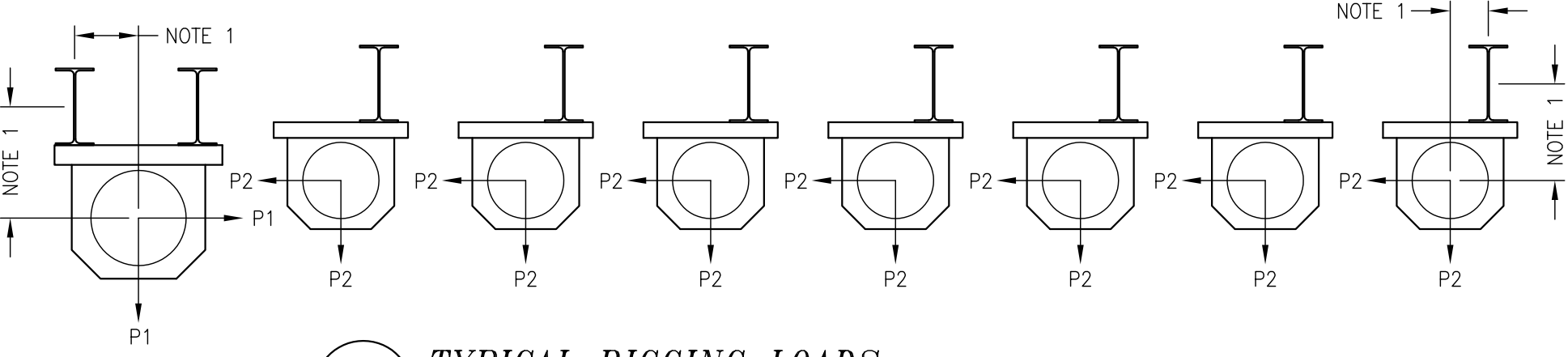
4 TYPICAL RIGGING LOADS PA-1 SCALE: NONE
