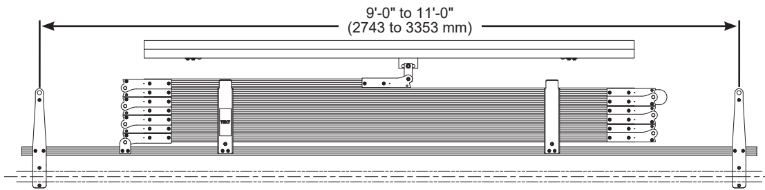
Pantograph Assembly
