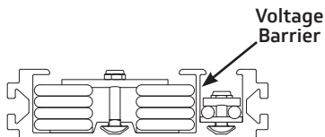
Arm Section View
