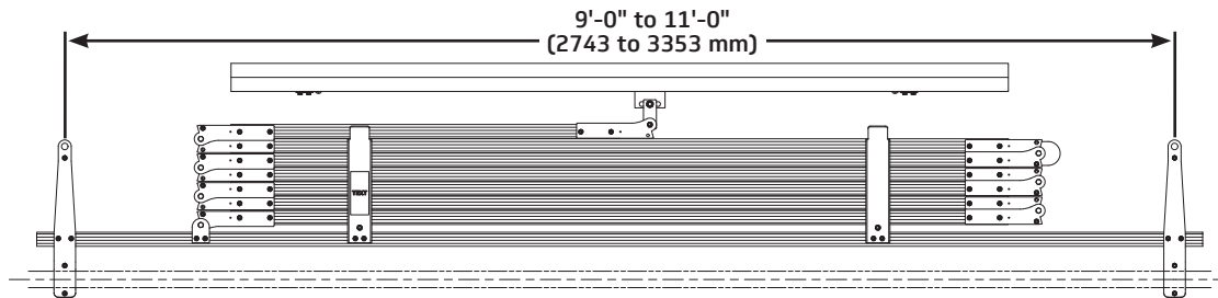
Pantograph Assembly
