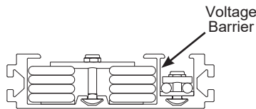
Arm Section View
