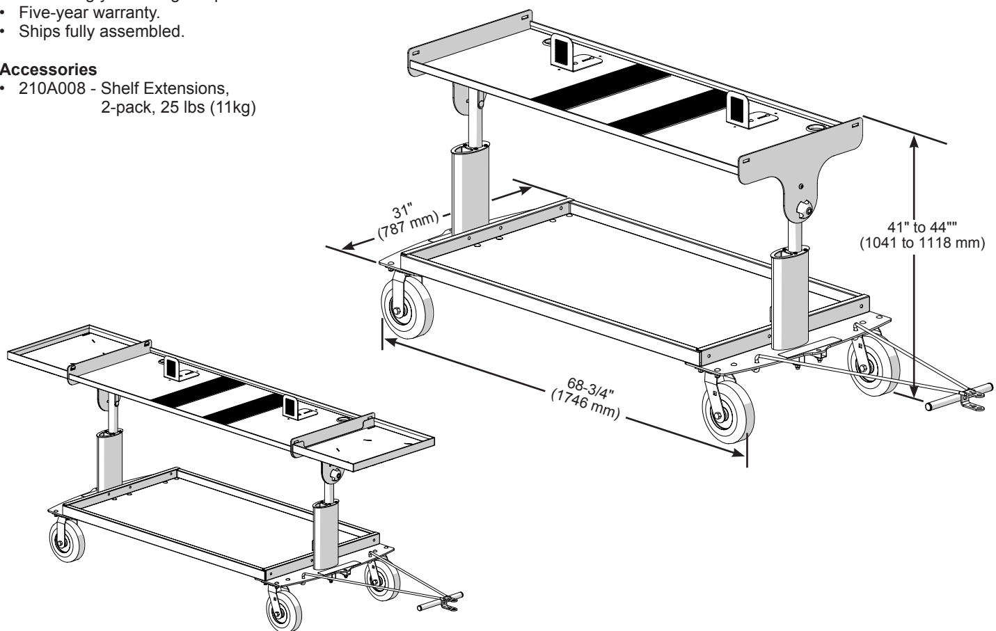
OnBoard Keyboard Cart shown with optional shelf extensions.
