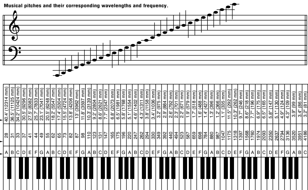
Musical pitches and their corresponding wavelengths and frequency.
