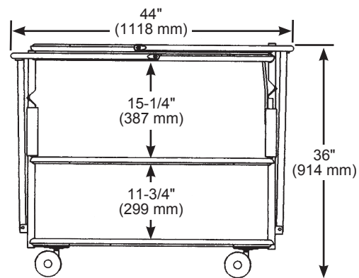
ORFFmobile in Folded Position
