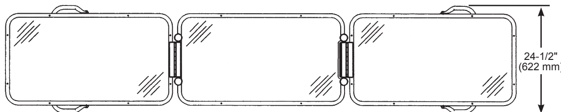
Top View
