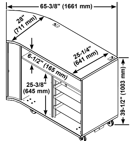
Left Curved Unit Assembly (Shown with Stereo Rack Option)
