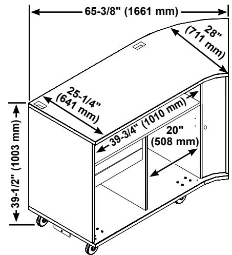
Right Curved Unit Assembly (Shown with Drawer Option)
