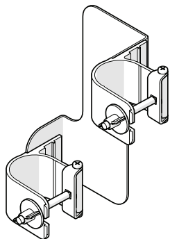
Right/Left 12" End Overlap Connector (left version shown)
