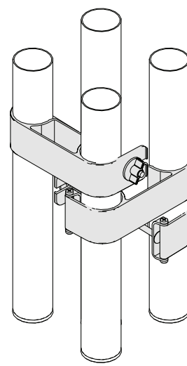
Leg Connector Securing Four Legs
