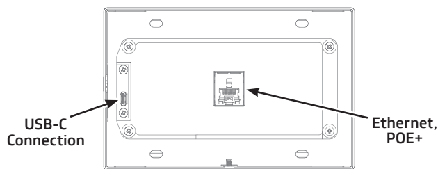
TS-1C Transcend Control Panel
